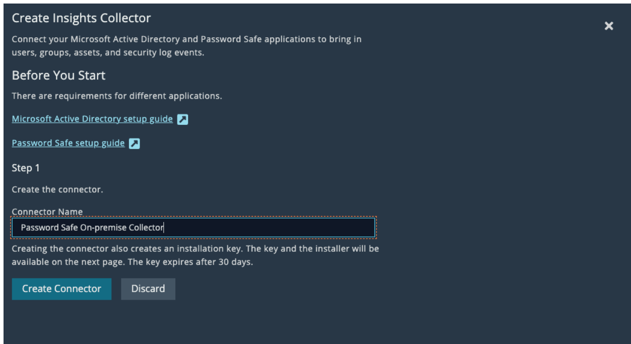
Figure 1 – Insights Collector
